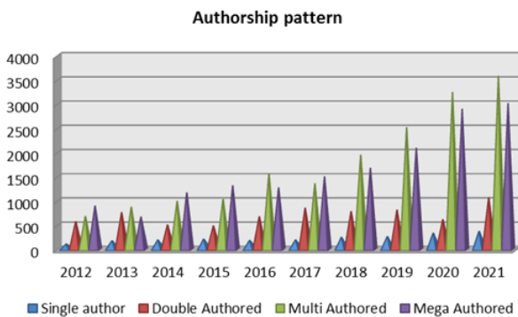
Fig. 4: Authorship pattern
