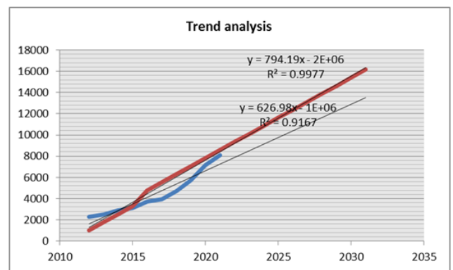
Fig. 2: Trend analysis
