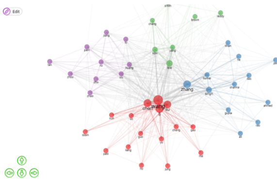
Fig. 7: Co-citation network
